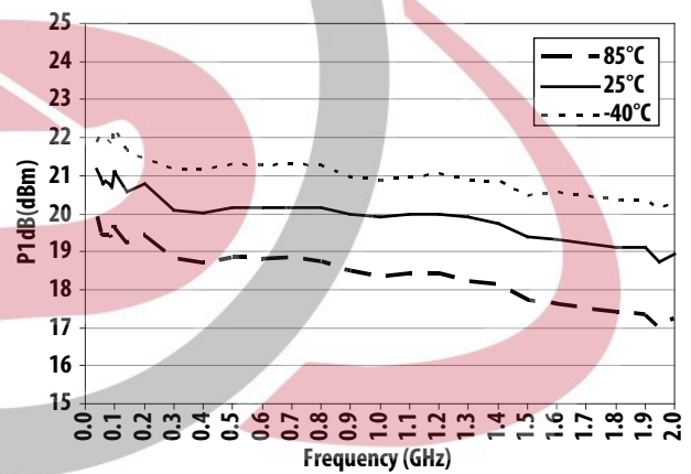
Figure 9. P1dB over Frequency and Temperature
